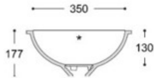
cross - section
