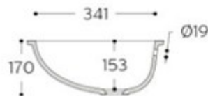
CROSS-SECTION
