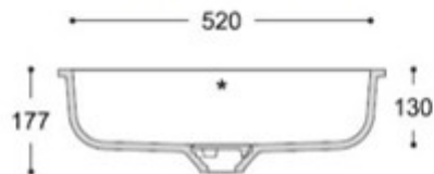
cross - section
