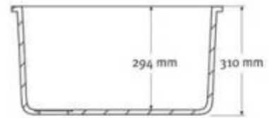
FRONT CROSS-SECTION
